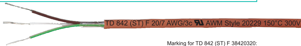
TD 842 (ST) F 20/7 AWG/3c AWM Style 20229 150°C 300V SAB BRÖCKSKES · D-VIERSEN · TD 842 (ST) F 20/7 AWG/3c AWM Style 20229 150°C 300V CE
